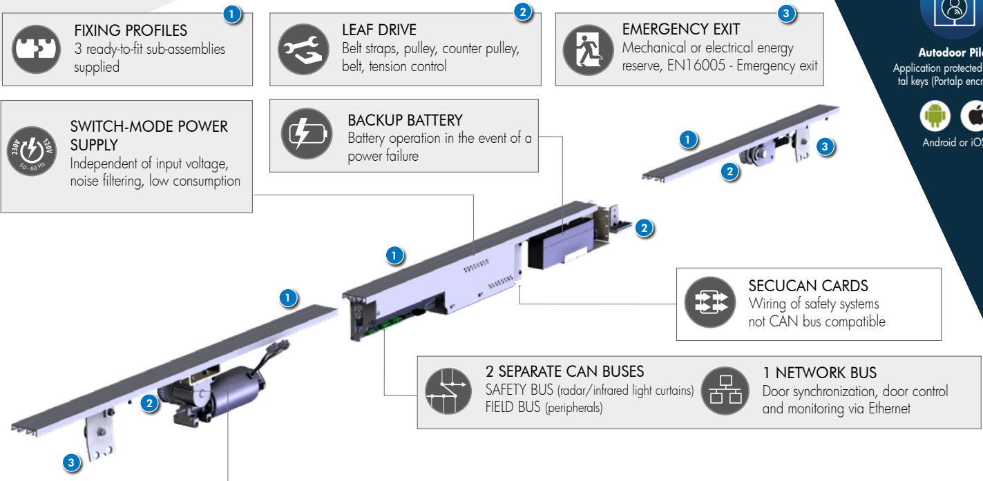
Compact RS operator integrated in the existing structure (Portalp or any other brand)
